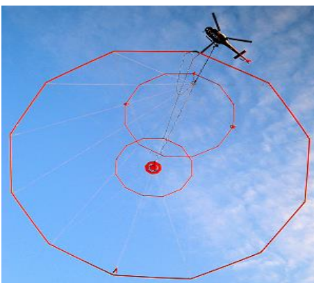
Geotech Ltd. VTEM Airborne Survey Array
